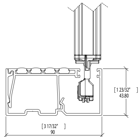
S1 Head and Sill Details
