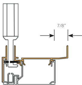
S4 Invisible sill (with 7/8" overhang)
